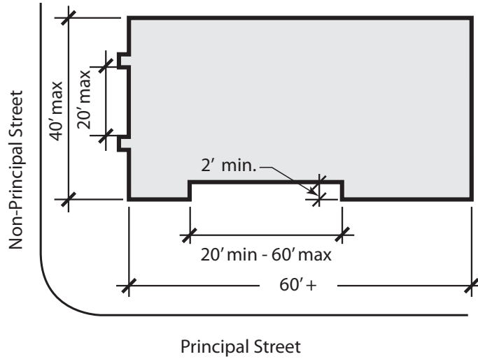
Figure 5-3: Diagram of building facade articulation.
