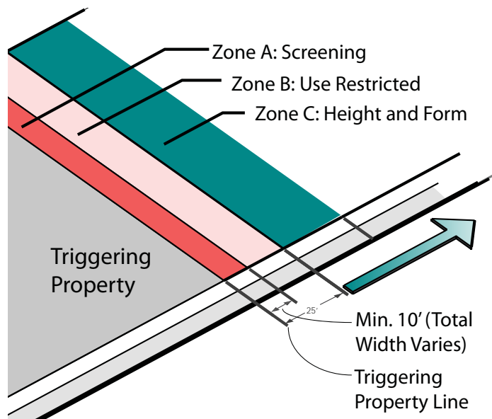
Figure 4-2: Transition Zone Locations This diagram illustrates the relationship between a triggering property, Zone A, Zone B, and Zone C.
