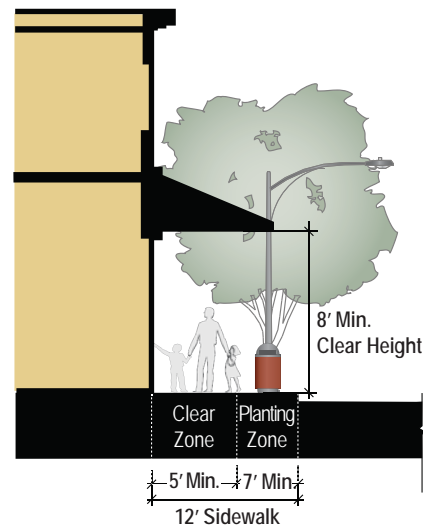
Figure 3-4: ERC Pedestrian Priority (PPC) & Urban Roadway (UR) Sidewalk Standards
